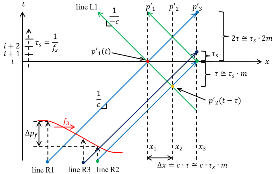
Figure 15. Characteristics of acoustic waves and the wave separation algorithm.
